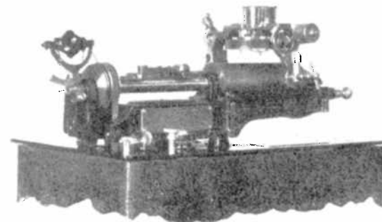
BETTINI'S SPEED INDICATOR IN POSITION.
